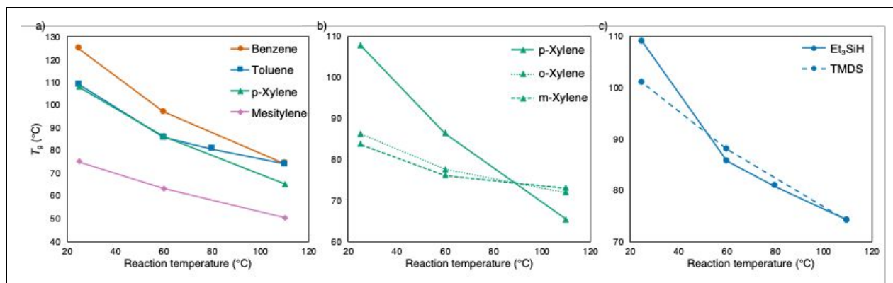
Fig. 3 T_g of polymer products from silylium catalyzed hydrodechlorination and Friedel-Crafts alkylation of PVC at 25, 60, 80 and 110 °C with: a) aromatic solvents with 0-3 methyl substituents, b) ortho, meta and para xylene, and c) comparisons between Et 3 SiH and TMDS as silane sources in toluene. All reactions were conducted with 0.25 mol% [Ph 3 C][B(C 6 F 5 ) 4 ], 2.53 mL aromatic solvent, 1.5 equiv. Et 3 SiH or 1.1 equiv. TMDS.
