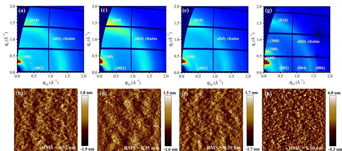
Fig. 2 2D-GIWAXS patterns and AFM height images ( 2\ \mu\text{m} \times 2\ \mu\text{m} ) of (a) and (b) cs-PyDT-BT-L , (c) and (d) cs-PyDT-BT-M , (e) and (f) cs-PyDT-BT-H , (g) and (h) as-PyDT-BT . The root-mean-square (RMS) surface roughness is also provided. The films of 2D-GIWAXS patterns were deposited by drop-casting and annealed at 150^\circ\text{C} for 30 min.
