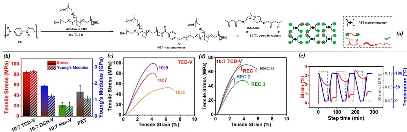
Fig. 14 (a) Vitrimers based on vinylogous urethane networks are synthesized via the crosslinking of PET macromonomers—efficiently depolymerized from PET through aminolysis—with AcAc crosslinkers. (b) The average tensile stress and Young's modulus for commercial PET and vitrimers incorporating different AcAc crosslinkers. (c) Tensile stress–strain curve of TCD-V vitrimers with different crosslinking densities. (d) Tensile stress–strain curves for the 10 : 7 TCD-V film after being repressed three times at 200 °C and 500 psi. (e) Consecutive cycles of shape memory behavior acquired from cyclic DMA experiments. Reproduced from ref. 63 with permission from John Wiley and Sons, copyright 2025.
