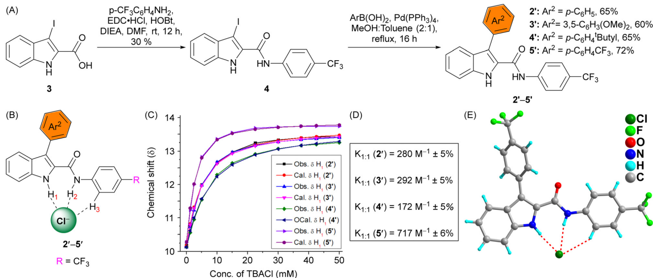
Fig. 2 Chemical synthesis of carriers 2'–5' (A). Chemical structure of the carriers showing binding interactions with the chloride anion (B). The plot of chemical shifts ( \delta ) of the H 1 proton vs. concentrations of TBACl added, fitted to a 1:1 binding model of BindFit for the active carriers 2'–5' (C). Binding constant values of carriers 2'–5' (D). (E) X-ray crystallographic structure of 5' with the chloride anion (D).
