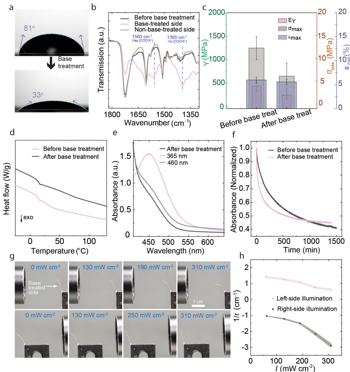
Fig. 4 After base treatment. (a) Contact angles, (b) FTIR spectra, and (c) Young's modulus ( E_y ), fracture strain ( \epsilon_{\max} ), and tensile strength ( \sigma_{\max} ) of the LCE before and after base treatment. The error bars represent the standard deviation obtained from n = 3 experiments. (d) DSC curves before and after base treatment, measured during the second cooling cycle with a rate of 10\text{ }^{\circ}\text{C min}^{-1} . (e) The n-\pi^* absorption band of the base-treated LCE (thickness 100\text{ }\mu\text{m} ) in the dark, after irradiation with 365\text{ nm} ( 15\text{ mW cm}^{-2} , 30\text{ s} ), and after subsequent irradiation with 460\text{ nm} ( 25\text{ mW cm}^{-2} , 30\text{ s} ). (f) Thermal cis-trans relaxation curves (monitored at 480\text{ nm} ) measured from a 20\text{ }\mu\text{m} thick LCE before and after base treatment. (g) Photographs of photochemical deformation of the base-treated LCE after UV illumination (different intensities) from either side, under 35\% relative humidity, and (h) corresponding bending curvatures.
