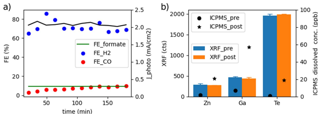
Fig. 10 (a) Stability test of \text{ZnGa}_2\text{Te}_4 without additives using a traditional H-cell at -0.8 V vs. RHE with periodic headspace measurements. Note that formate shown in the figure is the average over entire measurement. (b) Corrosion study by ICP-MS and XRF for pre- and post-PEC run samples.
