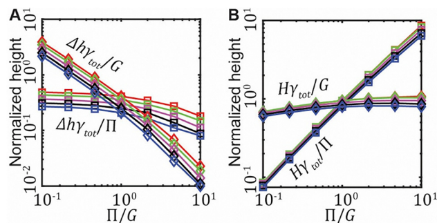
Fig. 2 (A) The osmocapillary length \gamma_{\text{tot}}/\Pi governs the phase separation size \Delta h . (B) The elastocapillary length \gamma_{\text{tot}}/G governs the solid height H red, green, magenta, black, and blue correspond to \gamma_{S2}/\gamma_{S1} = 1, 2, 3, 4, 5 .
