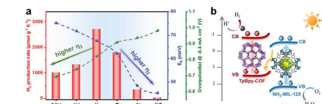
Fig. 9 (a) Photocatalytic H 2 production rate, E b and overpotential in the HER of UiO-66-NH 2 @Pt@UiO-66-X. 82 Copyright 2023, John Wiley and Sons. (b) Photocatalytic mechanism of the S-scheme heterojunction in NH 2 -MIL-125/TpBpy-COF for overall water splitting. 84 Copyright 2025, John Wiley and Sons.
