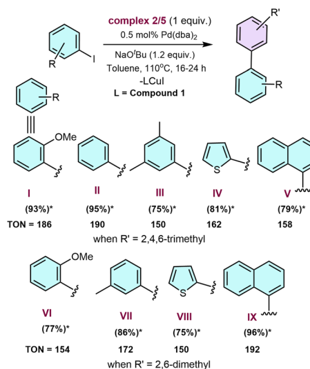
Scheme 7 Pd-catalysed \text{sp}^2\text{--sp}^2 C–C coupling reaction using 2 and 5 as an aryl transfer agent. *Isolated yields.
