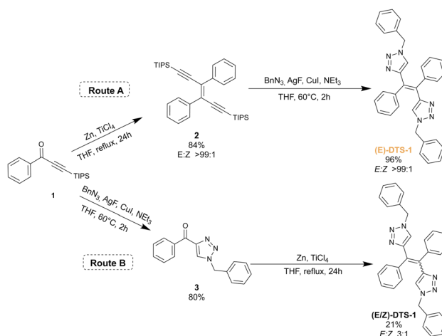
Fig. 2 Synthesis of DTS-1 following two different synthetic paths.
