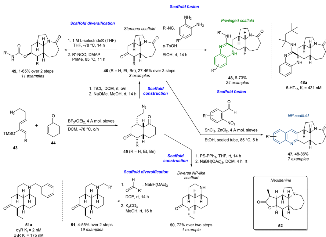
Scheme 3 Synthesis of stemona-inspired compounds and identification of 2-HT 1A ligand 48a and \sigma_1 R and \sigma_2 R ligand 51a. 85–87 L-selectride® = lithium tri-sec-butylborohydride, PS-PPh 3 = polystyrene bound triphenyl phosphine.
