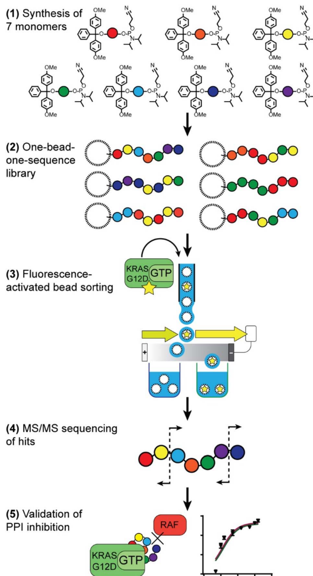
Fig. 1 Overview of route to selection of phosphoesters for PPI inhibition.
