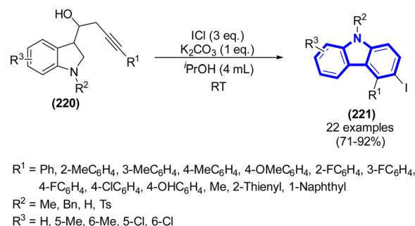
Scheme 59 Synthesis of carbazoles catalyzed by ICl and K₂CO₃.
