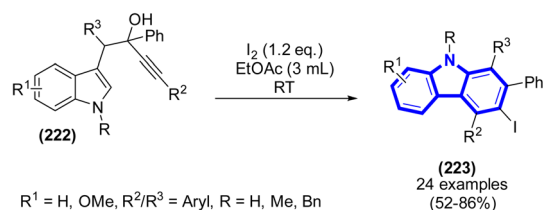
Scheme 60 Synthesis of 3-iodocarbazoles catalyzed by I₂.
