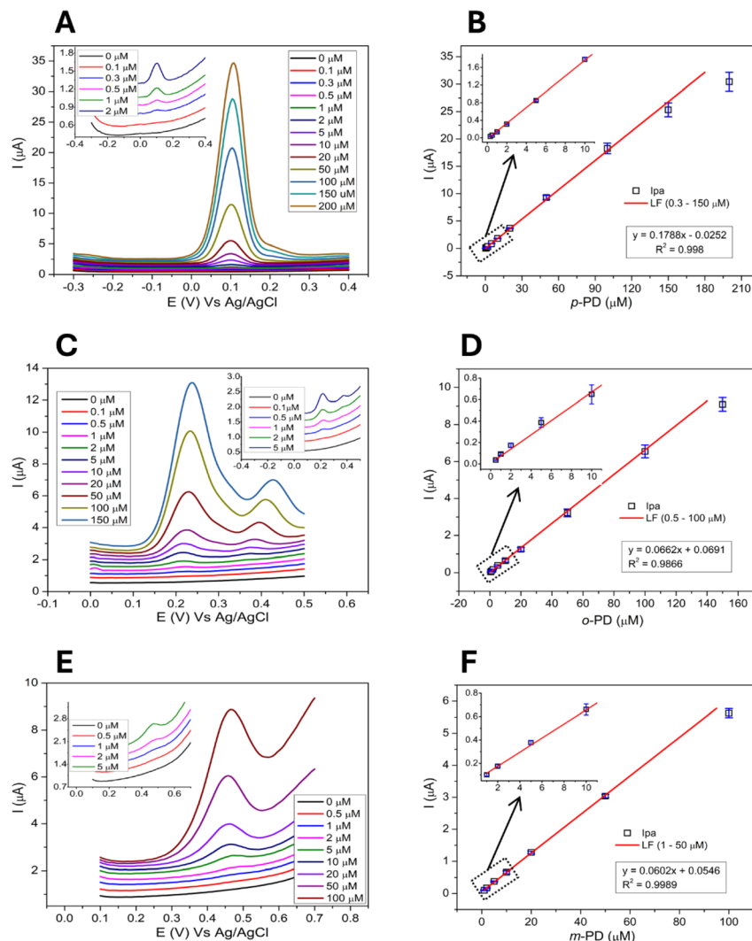
Fig. 7 Electrochemical response of the 1-SPGE for (A) p -PD, (C) o -PD, and (E) m -PD at different concentrations and the calibration curve (horizontally parallel), error bars represent the standard deviation among three replicates (SD, n = 3 ) (B) p -PD, (D) o -PD, and (F) m -PD respectively.
