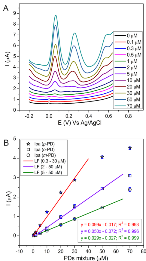
Fig. 8 Electrochemical response of 1-SPGE in the presence of p -PD, o -PD, and m -PD (A) and their calibration curves (B), error bars represent the standard deviation among three replicates (SD, n = 3 ).
