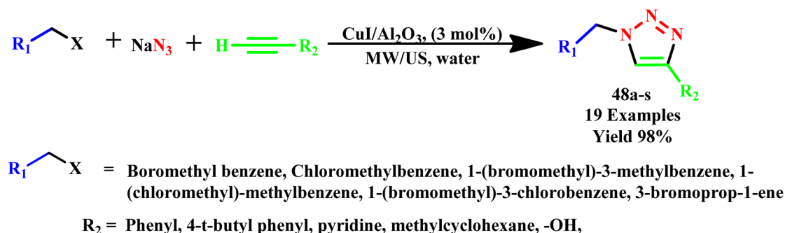
Scheme 37 Microwave-assisted synthesis of 1,4-disubstituted 1,2,3-triazoles (48a–s) via CuI on \text{Al}_2\text{O}_3 catalyzed. 76
