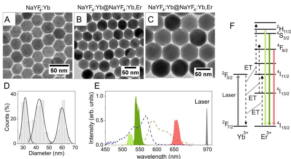
Fig. 1 (A) TEM image of the 32 nm \beta -NaYF 4 :Yb 0.20 core and \beta -NaYF 4 :Yb@NaYF 4 :Yb 0.20 ,Er 0.02 core-shell nanoparticles with different shell thicknesses: CS1, 5.5 nm (B) and CS2, 14 nm (C). (D) Size distribution of core ( 32 \pm 2 nm), and core-shell nanoparticles: CS1 ( 43 \pm 3 nm), and CS2 ( 60 \pm 3 nm), depicted in Fig. A, B, and C, respectively. (E) Green and red UCL emission spectrum of a NaYF 4 :Yb,Er UCNP s dispersion in DMSO at a concentration of 0.5 \text{ mg mL}^{-1} and excitation laser spectrum for a 967 nm CW laser power of 0.3 W ( 633 \text{ W cm}^{-2} ). Dashed lines show the absorption (left curve) and luminescence emission (right curve) spectra of the Cy3 dye FRET pair acceptor. (F) Energy level diagram for Yb 3+ and Er 3+ ions describing the processes that give rise to green and red UCL emission bands. The black dashed lines represent the Yb–Er energy transfer (ET) mechanism, whereas the green and red solid lines represent the two green and one red emissions, centered around 525 nm, 540 nm, and 655 nm, respectively.
