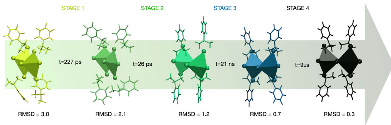
Fig. 2 Schematic illustration of S -MBA 2 PbI 4 configurations, highlighting various RMSD values obtained from the predicted free energy minima. The transition from a highly disordered ligands configuration toward the most chiral perovskite-like configuration is represented.
