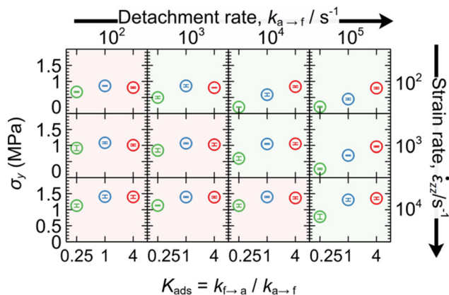
Fig. 12 Yield stress \sigma_y as a function of the detachment rate k_{a \rightarrow f} , elongation rate \dot{\epsilon}_{zz} and adsorption constant K_{\text{ads}} = k_{f \rightarrow a} / k_{a \rightarrow f} = 1/4 (green), 1 (blue) and 4 (red). Scenarios where \dot{\epsilon}_{zz} is smaller (larger or equal) than k_{a \rightarrow f} are indicated with green (red) background. The error bars correspond to the standard deviation from three individual experiments.
