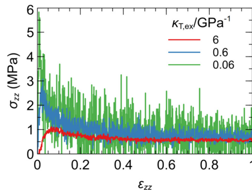
Fig. 13 Stress–strain curve from a tack experiment with \dot{\epsilon}_{zz} = k_{a \rightarrow f} = 10^5 \text{ s}^{-1} and K_{\text{ads}} = 1 . Red curve illustrates a case using the default parameters in Table 1. Blue/green curve illustrates the impact of decreasing compressibility by a factor of 10/100 upon multiplying the characteristic pressure P^* by 10/100, respectively.
