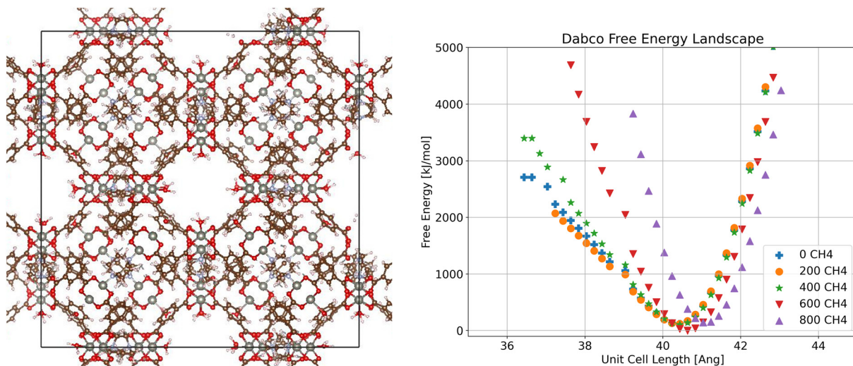
Fig. 2 Visualization of crystalline ZnMOP-Dabco system and free energy landscape of the system as a function of unit cell side length and methane loading in molecules/unit cell.
