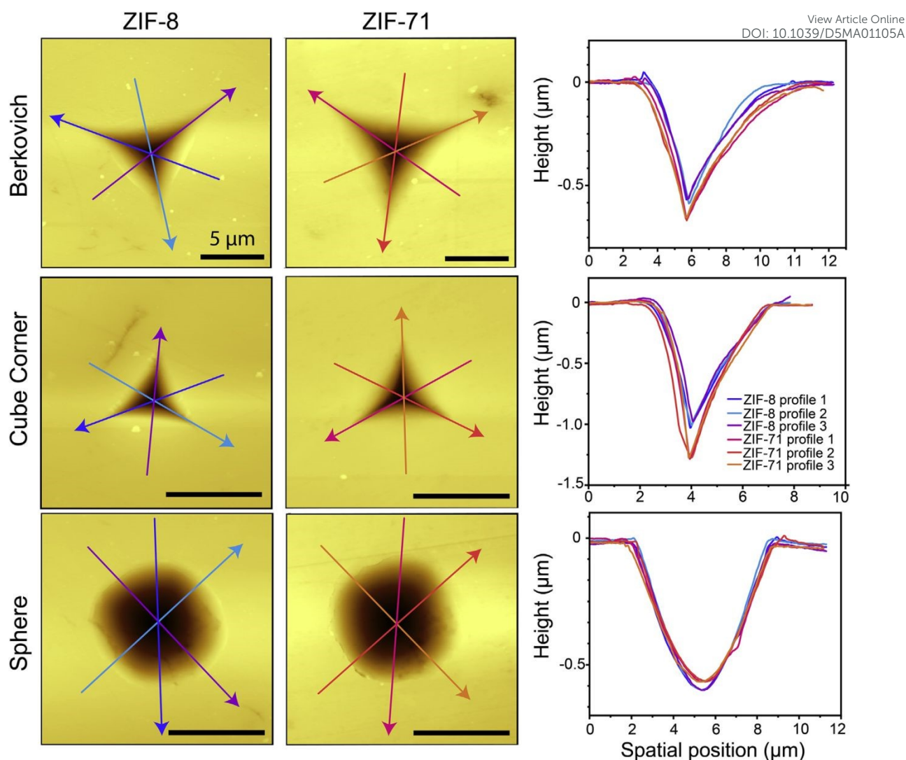
Figure 23: AFM height topography of the residual indents of Berkovich, cube corner, and spherical indentations for ZIF-8 and ZIF-71 monoliths. 35 Reproduced with permission from reference 35, Copyright (2022) Elsevier B. V.
