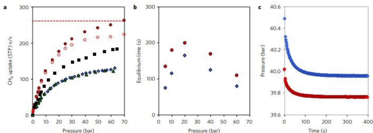
Figure 294: Gas adsorption in HKUST-1. a) Comparison of absolute volumetric methane adsorption isotherms at 298 K on \text{monoHKUST-1} (red filled circles), excess volumetric uptake on \text{monoHKUST-1} (red open circles), HKUST-1 pellets under hand packing (blue diamonds), HKUST-1 pellets packed under 27.6 MPa (black squares), and HKUST-1 pellets under 68.9 MPa (green triangles). b) Equilibrium time of methane adsorption at 298 K as a function of equilibrium pressure, and c) decay of pressure with time at 40 bar for \text{monoHKUST-1} (blue diamonds) and \text{powdHKUST-1} (red circles). 32 Reproduced with permission from reference 32. Copyright (2017) Springer Nature Limited.
