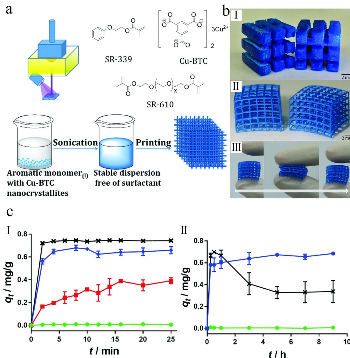
Figure 13. Digital Light Processing (DLP) of HKUST-1 composites: a) schematic of the DLP strategy and material chemistries, b) photographs of the resulting flexible 3D-printed monoliths, and c) evaluation of their methylene blue (MB) adsorption performance over time. 64 Reproduced from reference 64, under the terms of Creative Commons (CC BY) licence.
