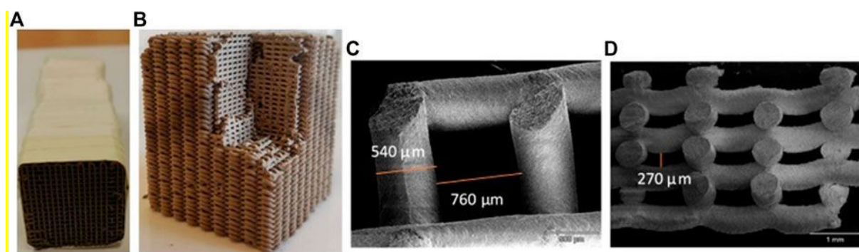
Figure 5: 3D printed ZIF-8 monolith. A) Monolith used for breakthrough experiments. Several pieces were stacked and held together with Teflon tape. (B) Side view showing the presence of channels in the radial direction. (C) Scanning electron microscopy-picture of the top-view of the monolith. (D) Scanning electron microscopy-picture of side view visualizing the radial gaps present in the structure. 53 Reproduced with permission from reference 53 , under the terms of the Creative Commons Attribution License (CC BY).
