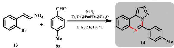
Scheme 6 \text{Fe}_3\text{O}_4 @poly( m -phenylenediamines)@ \text{Cu}_2\text{O} catalysed synthesis of quinazolinones (Rawat et al. ).
