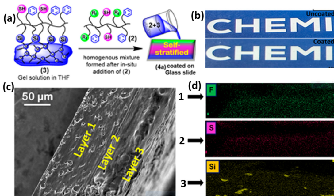
Fig. 15 (a) Graphical representation of the formation of self-stratified polymers based on fluorosul/thiol/siloxane, (b) comparison of uncoated and coated polymers on glass, (c) SEM images of a cross-section of the cured film, and (d) corresponding EDX dot mapping of three positions. Reproduced with permission; 97 Copyright 2023, ACS.
