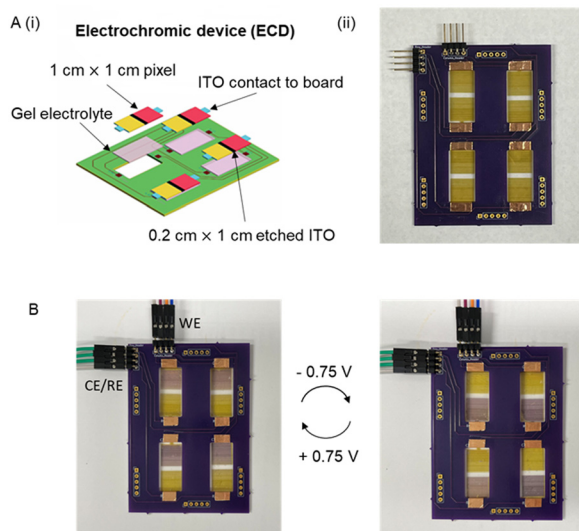
Fig. 3 Integration of the PGE with arrayed pixels. (A)(i) Schematic of the board and pixel integration scheme and (ii) image showing the integrated pixels (each consisting of two 1 cm 2 printed squares) with the PGE on the printed circuit board before polarization. (B) Chronoamperometric application of a \pm 0.75 V DC potential (200 s per cycle) demonstrated the capability for synchronized colour change. Within the pixel array.
