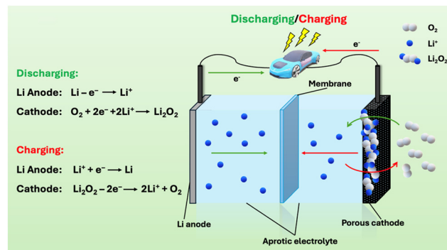
Fig. 1 Structure and working principles of aprotic LOBs. During discharge, \text{Li}^+ ions move from the anode zone to the cathode zone, where \text{O}_2 molecules are reduced on the cathode and then combine with \text{Li}^+ to form insoluble \text{Li}_2\text{O}_2 . During charge, \text{Li}^+ ions move backwards, and \text{Li}_2\text{O}_2 is oxidized to \text{O}_2 , ideally.
