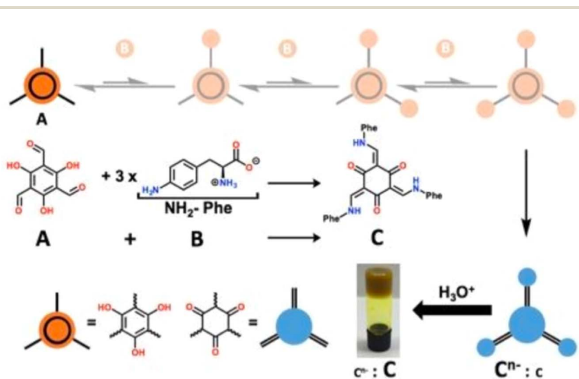
Fig. 2 Synthetic scheme showing the reaction between A and B in alkaline water, pH 8, which gives rise to the formation of deprotonated non supramolecular fibre structure C^{n-} . Subsequent acidification of C^{n-} results in protonation and concomitant formation of the low molecular weight gelator C . Reproduced from https://doi.org/10.1039/D5FD00016E with permission from the Royal Society of Chemistry.
