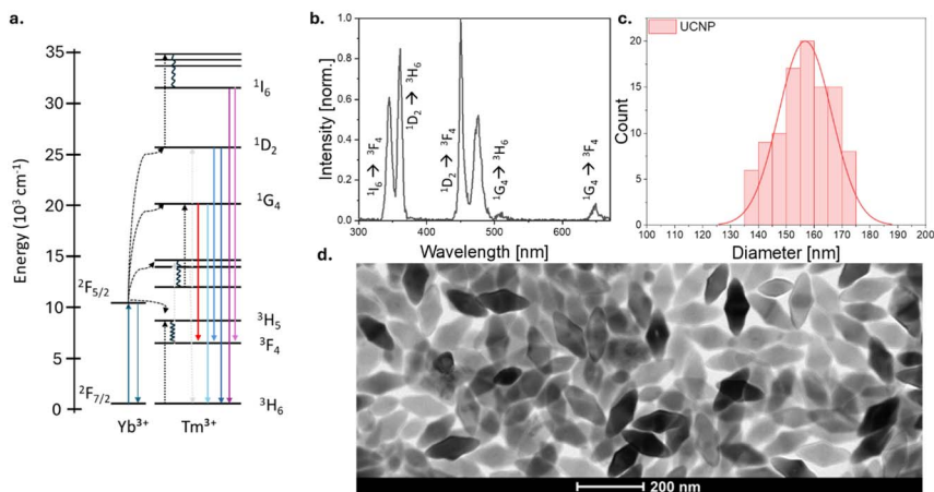
Fig. 2 (a) Energy-level diagram illustrating the upconversion mechanism facilitated by \text{Yb}^{3+} and \text{Tm}^{3+} ions in the UCNP. The UCNPs are composed of \text{LiYF}_4 doped with 0.5 mol% \text{Tm}^{3+} and 25 mol% \text{Yb}^{3+} . (b) Emission spectrum of the UCNPs, showing efficient generation of UV light upon excitation at 980 nm. (c) Size distribution of the synthesized UCNPs, revealing a particle diameter of 135–175 nm. (d) Transmission electron microscopy (TEM) image of diamond-shaped UCNPs. 29,30
