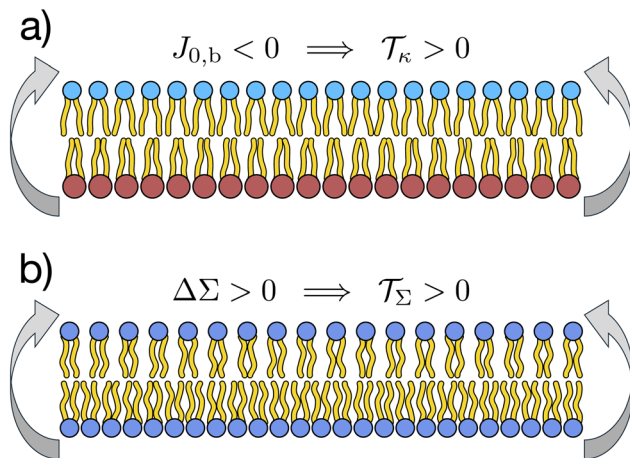
Fig. 2 Clarifying the sign of the torque, \mathcal{F} = \mathcal{F}_{\kappa} + \mathcal{F}_{\Sigma} . (a) The torque due to lipid curvature, \mathcal{F}_{\kappa} , strives to bend the membrane up when the spontaneous bilayer curvature is negative, J_{0,\text{b}} < 0 , i.e. when the upper leaflet has a more negative spontaneous curvature than the lower one. (b) The torque due to differential stress, \mathcal{F}_{\Sigma} , strives to bend the membrane up when the differential stress is positive, \Delta \Sigma > 0 , i.e. when the upper leaflet is under excess tension.
