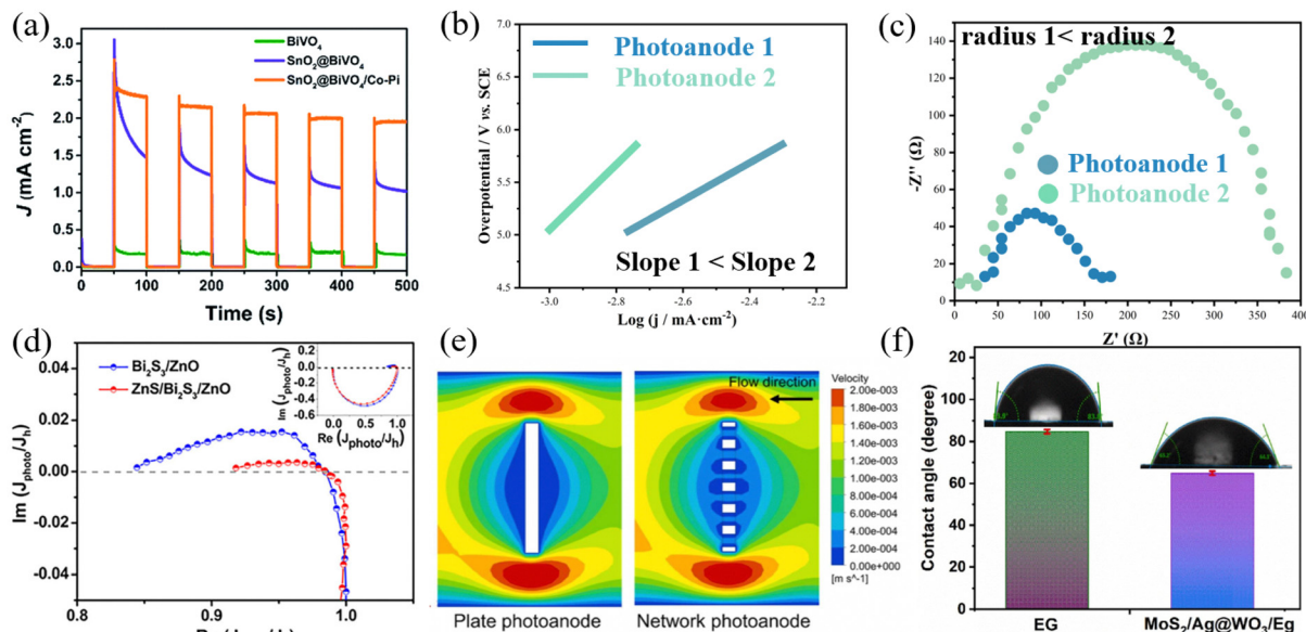
Fig. 8 Techniques for characterizing interfacial reaction processes: (a) photocurrent–time curves of pristine \text{BiVO}_4 , \text{SnO}_2 @ \text{BiVO}_4 , and \text{SnO}_2 @ \text{BiVO}_4 /Co–Pi photoanodes, reprinted with permission from ref. 86, Copyright (2019) Royal Society of Chemistry. Schematic diagram of (b) Tafel curves and (c) Nyquist plots (where it is assumed that photoanode 1 has faster interfacial charge transfer kinetics than photoanode 2). (d) IMPS Nyquist plots of the \text{Bi}_2\text{S}_3 /ZnO NRA and \text{ZnS}/\text{Bi}_2\text{S}_3 /ZnO NRA, respectively, reprinted with permission from ref. 54, Copyright (2022) American Chemical Society. (e) CFD simulations of the flow velocity in the plate and network electrode in flowing water, reprinted from ref. 46, Copyright (2022), with permission from Elsevier. (f) Contact angle of EG and \text{MoS}_2/\text{Ag}/\text{WO}_3/\text{EG} photoanodes, reprinted from ref. 124, Copyright (2023), with permission from Elsevier.
