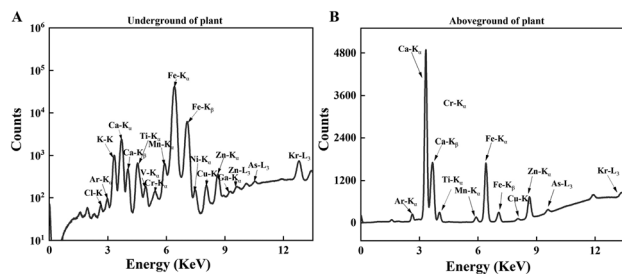
Fig. 4 The SR-μXRF spectrum showing the presence of mineral elements in the (A) underground and (B) aboveground parts of plant.
