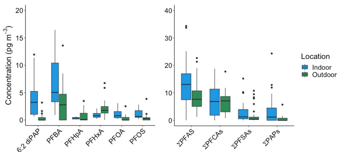
Fig. 2 Distributions of PFAS with DF > 50% on indoor front and/or outdoor filter-collected \text{PM}_{2.5} for all homes (left image) and \Sigma PFAS, \Sigma PFCAs, \Sigma PFSA, \Sigma PAPs for indoor front and outdoor filter-collected \text{PM}_{2.5} (right image). Concentrations are field blank subtracted. Note: the (left image) y-axis was limited to 20 \text{ pg m}^{-3} for better data visualization. PFBA had three additional outliers ( 50.1 , 82 , 119 \text{ pg m}^{-3} ). The (right image) y-axis was limited to 40 \text{ pg m}^{-3} . There were three additional outliers for \Sigma PFAS indoor front filter ( 61.1 , 88.8 , 135 \text{ pg m}^{-3} ) and three for \Sigma PFCAs indoor front filter ( 50.8 , 82.5 , 119.4 \text{ pg m}^{-3} ).
