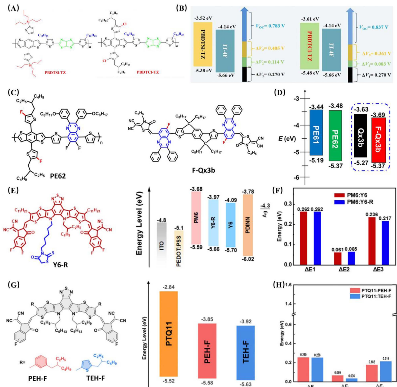
Fig. 5 (A) Chemical structures of PBDSi-TZ and PBDCI-TZ; (B) energy loss of devices based on PBDSi-TZ:IT-4F and PBDCI-TZ:IT-4F. 86 Copyright 2020 WILEY-VCH. (C) Chemical structures of PE62 and F-Qx3b; (D) energy levels of PE62 and F-Qx3b. 87 Copyright 2021 Elsevier. (E) Chemical structure of Y6-R and energy level of its device; (F) energy loss of devices based on PM6:Y6 and PM6:Y6-R. 91 Copyright 2025 American Chemical Society. (G) Chemical structures and energy levels of PEH-F and TEH-F; (H) energy loss of devices based on PTQ11:PEH-F and PTQ11:TEH-F. 92 Copyright 2025 Royal Society of Chemistry.
