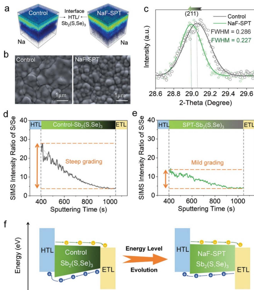
Fig. 3 (a) 3D-SIMS images of Na. (b) Surface SEM images. (c) Enlarged XRD spectra of 2-theta from 28.6^\circ to 29.8^\circ . (d and e) SIMS intensity ratios of S/Se in \text{Sb}_2(\text{S,Se})_3 films. (f) Schematic diagram of energy levels of \text{Sb}_2(\text{S,Se})_3 devices with or without NaF-SPT. Reproduced with permission from ref. 27 with permission from Wiley, copyright 2022.
