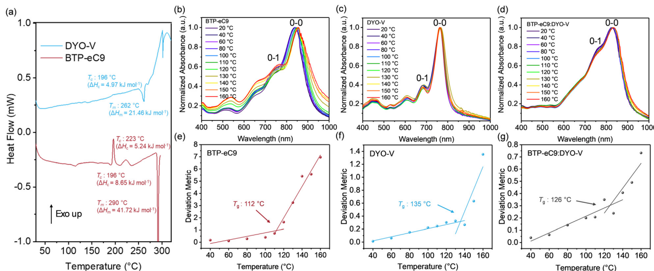
Fig. 2 (a) DSC thermograms of BTP-eC9 and DYO-V, collected from the first cycle with a 10^\circ\text{C min}^{-1} heating rate. (b)–(d) Temperature-dependent absorption spectra and (e)–(g) deviation metrics obtained from the temperature-dependent absorption of the BTP-eC9, DYO-V and BTP-eC9:DYO-V films.
