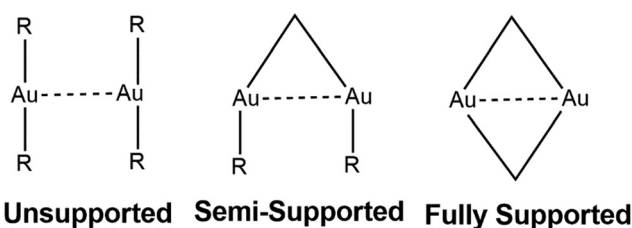
Fig. 1 Visual representation of unsupported, semi-supported, and fully supported aurophilic interactions.
