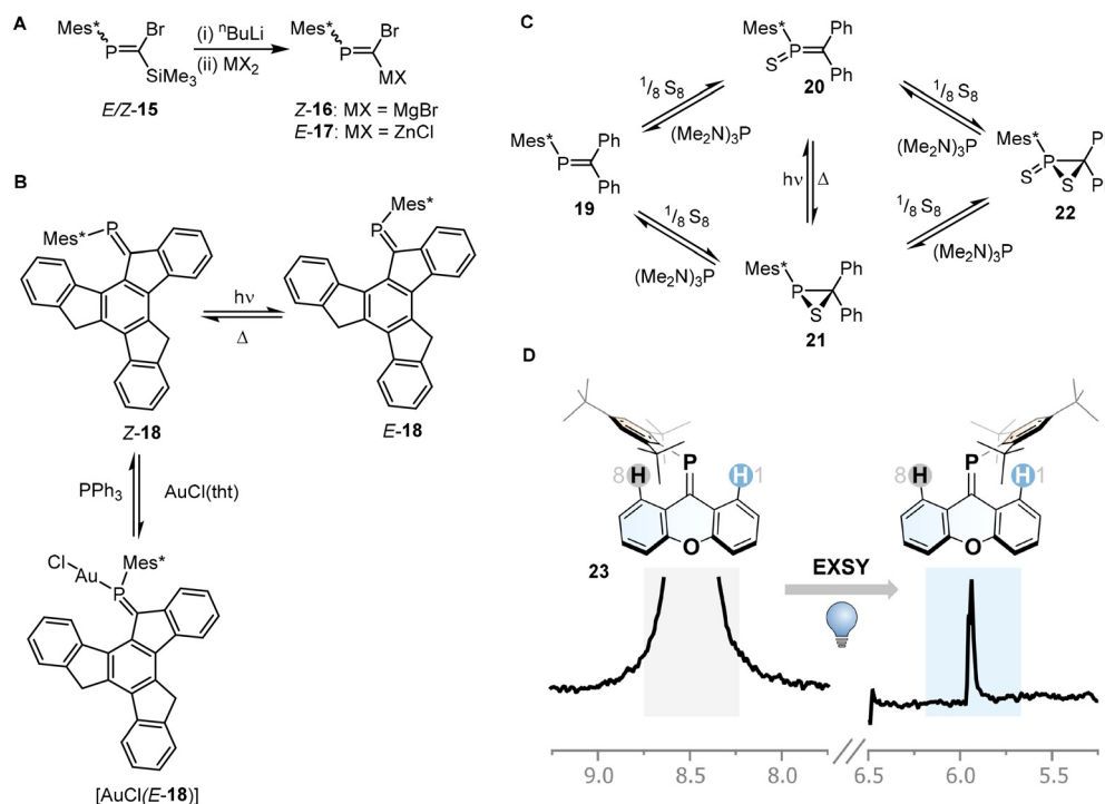
Fig. 4 A and B. Metal mediated isomerisation in phosphaaalkenes 15 and 18 ; C. sulfurization induced isomerisation in phosphaaalkene 19 ; D. degenerate isomerism in phosphaaalkene 23 . \text{Mes}^* = 2,4,6\text{-}t\text{Bu}_3\text{C}_6\text{H}_2 ; image is reproduced from Angew. Chem., Int. Ed. , 2025, 64 , e202419943 under the CC-BY license.
