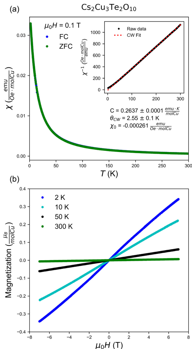
Fig. 8 (a) Magnetic susceptibility measurements of \text{Cs}_2\text{Cu}_3\text{Te}_2\text{O}_{10} were performed under ZFC and FC conditions with an applied external field of \mu_0H = 0.1 T. Inverse magnetization (inset) shows Curie–Weiss-like behavior with \theta_{CW} = 2.55 \pm 0.1 K, indicating net ferromagnetic interactions. (b) Isothermal magnetization data for \text{Cs}_2\text{Cu}_3\text{Te}_2\text{O}_{10} were collected at temperatures of T = 2, 10, 50 , and 300 K, within the external magnetic field range of \mu_0H = \pm 7 T.
