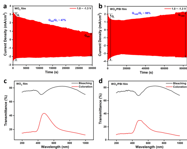
Fig. 3 Chronoamperometry curves of WO 3 (a) and WO 3 /PBI hybrid films (b) in 1 mol L -1 LiClO 4 /PC electrolyte. Optical transmittance difference ( \Delta T = T_{\text{colored}} - T_{\text{bleached}} ); corresponding UV-vis transmittance spectra of the WO 3 (c) and WO 3 /PBI hybrid films (d) in colored and bleached states between 200 nm and 1000 nm.
