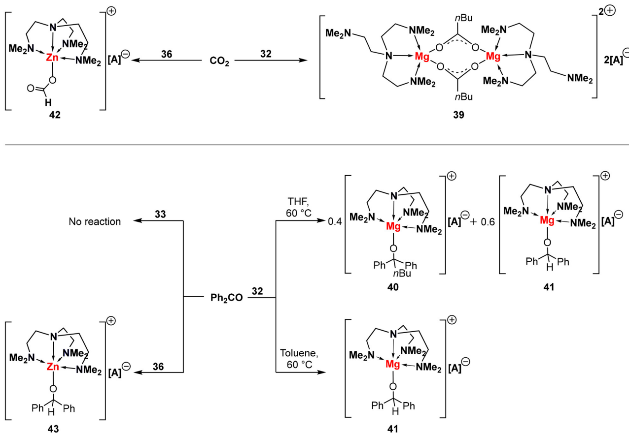
Scheme 10 Reactivity of the n -butylmagnesium cation 32 and the hydrido-zinc cation 36 towards electrophiles like \text{CO}_2 (top) and \text{Ph}_2\text{CO} (bottom).
