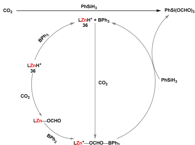
Scheme 11 Proposed catalytic cycle for the selective hydrosilylation of \text{CO}_2 using \text{PhSiH}_3 in the presence of the hydrido-zinc cation 36 and triphenylborane.
