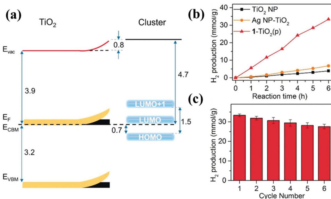
Fig. 6 (a) Schematic energy diagram of TiO 2 before (black) and after (orange) deposition of NCs, (b) hydrogen evolution activity under UV/vis light irradiation, and (c) recyclability test of the composite. Reproduced with permission from ref. 59. Copyright 2020 Wiley-VCH.
