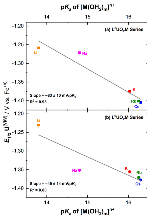
Fig. 7 Plot of E_{1/2}(\text{U}^{\text{VI}}/\text{U}^{\text{V}}) vs. \text{pK}_a of [\text{M}(\text{H}_2\text{O})_6]^{n+} for L 5 UO 2 M complexes (a, upper panel) and L 6 UO 2 M complexes (b, lower panel).
