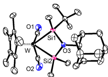
Fig. 2 Crystal structure of Cp^*W(CO)_2\{Me_2Si\cdots O(Ad)\cdots Si^tBuMe\} ( 5 ). Selected interatomic distances (Å): W–Si1 2.535(3), W–Si2 2.500(3), Si1–O3 1.871(8), Si2–O3 1.817(8). Hydrogen atoms have been omitted for clarity.
