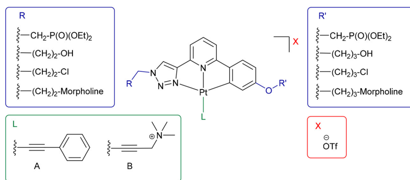
Chart 2 Structural composition of the Pt(II) complexes. The basic structure of the ligand (black), the functionalization sites R and OR' (blue), the auxiliary ligand L to be varied (green), and the respective counterion (red) are highlighted in a color code.
