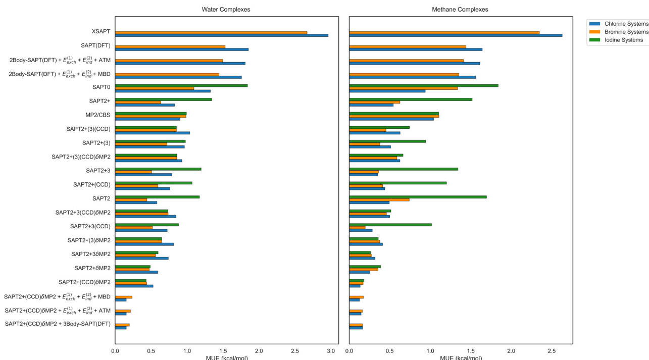
Fig. 9 Mean unsigned errors (MUE, \text{kcal mol}^{-1} ) of the total (two-body plus three-body) interaction energy estimates relative to the benchmark CCSD(T)-level complete E_{\text{int}} values, grouped by the identity of the halogen bond donor. For consistency between different methods, the data with chlorine and bromine as the XB donor do not contain the 6 systems (3 with water and 3 with methane) involving iodine in a different capacity (for which the XSAPT and three-body SAPT(DFT) data are not available).
