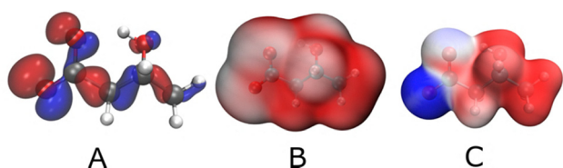
Fig. 2 (A) HOMO, (B) average local ionisation energy (ALIE) and (C) condensed Fukui ( f^- ) function for (R)-3-hydroxybutyrate. For (B) and (C) the colour progression from red to white to blue indicates increasing electron density.
