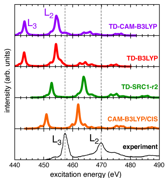
Fig. 1 Direct relation between the accuracy of TD-DFT calculations and the fraction of exact exchange, for Ti L_{2,3} -edge spectra of \text{TiCl}_4 . Shown are four different TD-DFT approaches along with CAM-B3LYP/CIS, in comparison to an experimental spectrum from ref. 121. All calculations used the def2-TZVPD basis set and include 200 singlet and 200 triplet basis states. Individual transitions were broadened using a Lorentzian function with FWHM = 0.3 eV.
