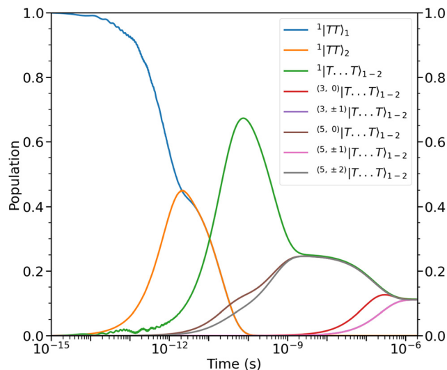
Fig. 4 Populations as a function of time of the intrachain states, |1^1\text{TT}\rangle_1 and |1^1\text{TT}\rangle_2 , and interchain states, |^{(2S+1)M_S}\text{T}\cdots\text{T}\rangle_{1-2} . The dynamics can be divided into four time regimes, which are described in the main text. States of same spin and magnitude of M_S are populated simultaneously. Note that the rate of population of the triplet and quintet states with M_S = \pm 1 are similar enough that the two lines corresponding to those populations (purple and pink) overlap. At ca. 2 \mu\text{s} the nine lowest energy levels (illustrated in Fig. 3) are equally populated.
