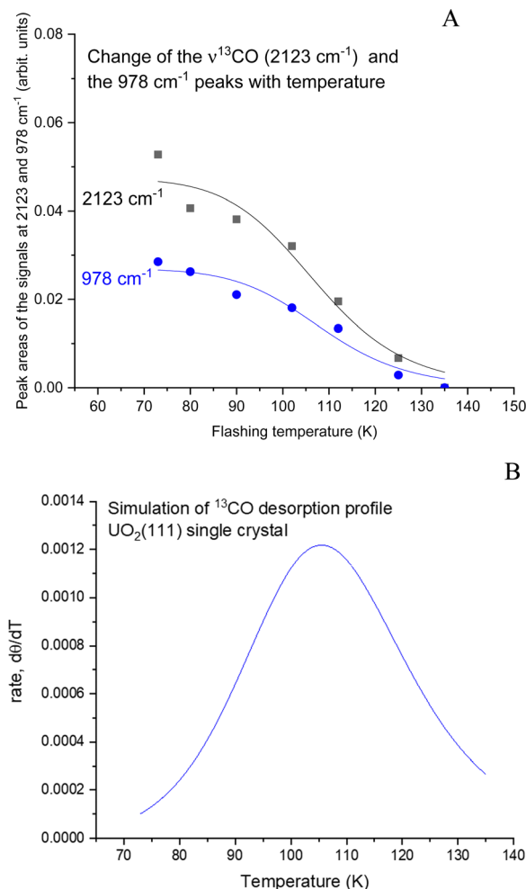
Fig. 6 (A) Changes in the peak areas of the signals at 2123 and 978 cm -1 with temperature. The peak area of the signal at 978 cm -1 is the sum of both the positive and negative peaks. The fitting is a Langmuir-type function ( Y = 1/(a + bx^{-1}) ) with a , b , and c being constants. (B) Derivative of the fitted function in (A) representing the desorption rate of CO from \text{UO}_2(111) single crystal. The maximum temperature of 105 K gives a desorption energy of 26–28 kJ mol -1 (270–290 meV).
