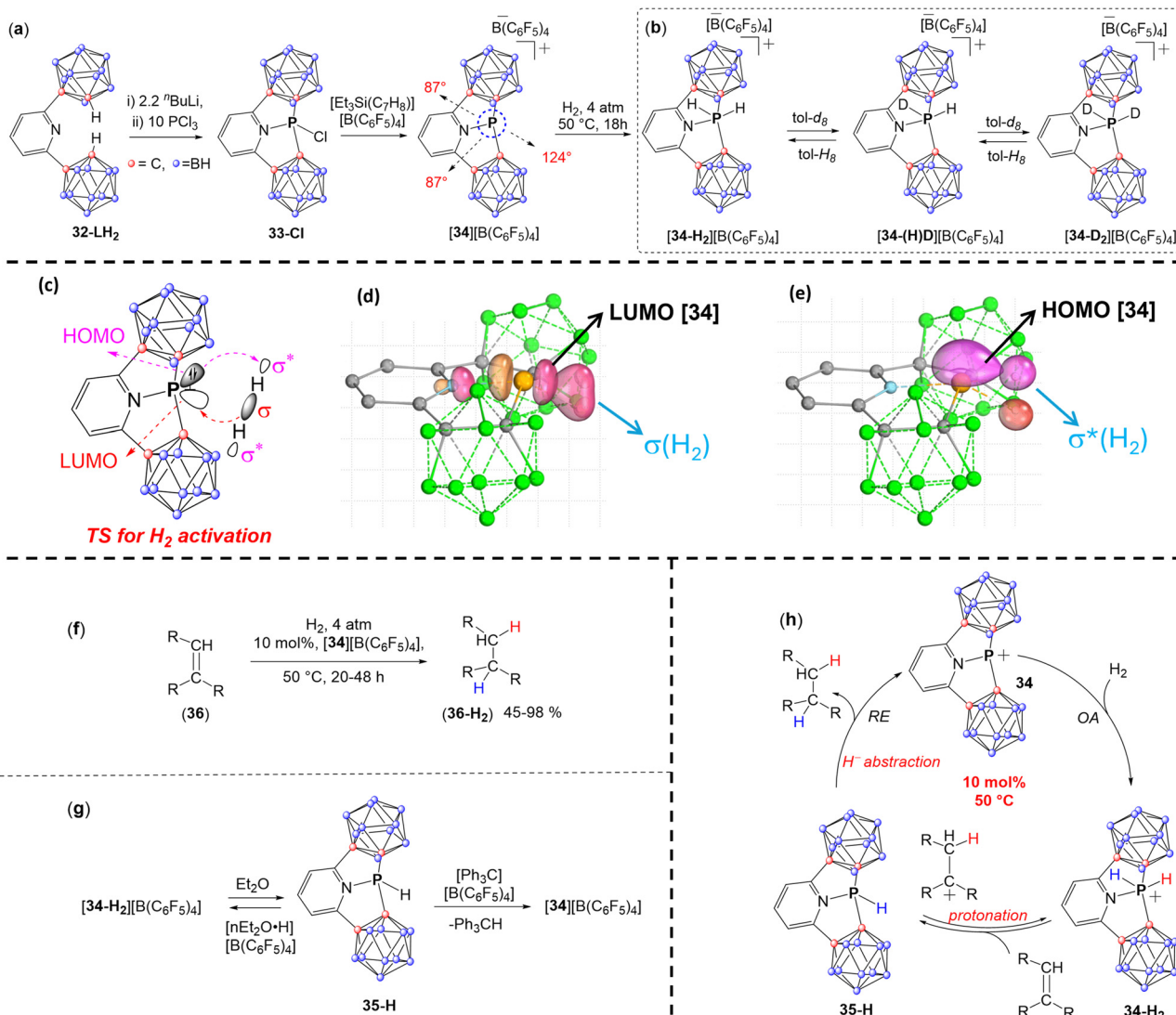
Fig. 13 Synthetic scheme for (a) the synthesis of [34][\text{B}(\text{C}_6\text{F}_5)_4] ; (b) the activation of dihydrogen by [34][\text{B}(\text{C}_6\text{F}_5)_4] and the exchange reaction between the H–H bond and D atom between [34\text{-H}_2][\text{B}(\text{C}_6\text{F}_5)_4] and toluene- \text{d}_8 and vice-versa; (c) schematic representation to show electrophilically driven activation of the H–H bond by 34 ; (d) \sigma -bond of \text{H}_2 approaching the P-centre from the direction of the LUMO of 34 ; (e) followed by the interaction of the HOMO of the P-centre with the LUMO ( \sigma^* ) of \text{H}_2 ; (f) [34][\text{B}(\text{C}_6\text{F}_5)_4] catalyzed hydrogenation reactions of unsaturated C–C species; (g) equilibrium of [34][\text{B}(\text{C}_6\text{F}_5)_4] with 35\text{-H} and reaction of 35\text{-H} with [\text{Ph}_3\text{C}][\text{B}(\text{C}_6\text{F}_5)_4] ; and (h) the proposed catalytic cycle.
