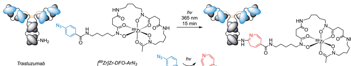
Scheme 3 Photoradiosynthesis to label a monoclonal antibody with a positron-emitting ^{89}\text{Zr} -desferrioxamine complex via light-induced activation of a \text{ArN}_3 group. Trastuzumab is linked in a one-pot photoreaction to [\text{}^{89}\text{Zr}]\text{ZrDFO-ArN}_3 with high isolated and decay-corrected radiochemical yields and radiochemical purities. 28,53,54
