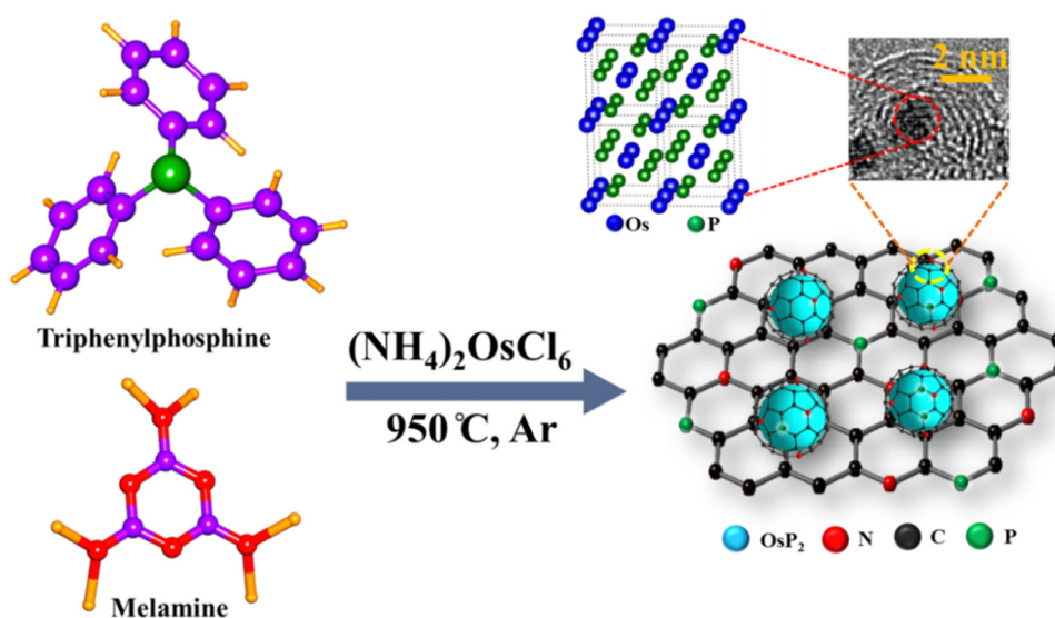
Fig. 5 Synthesis of \text{OsP}_2@NPC using TPP as a phosphidating agent. Reproduced with permission from ref. 65. Copyright 2019 Royal Society of Chemistry.
